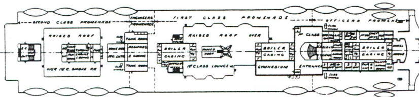
BOAT DECK
