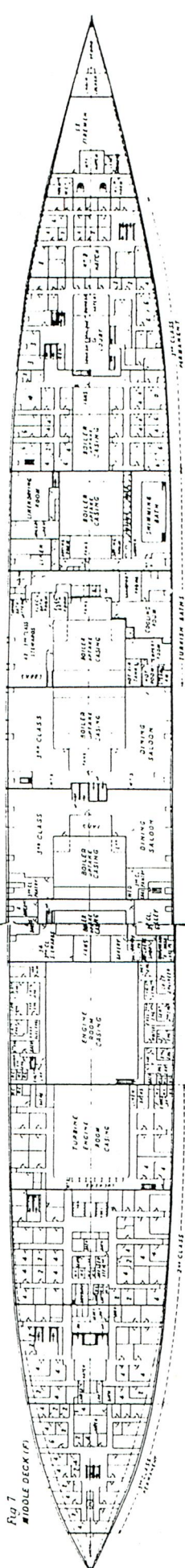
Fig. 8. LOWER DECK.
