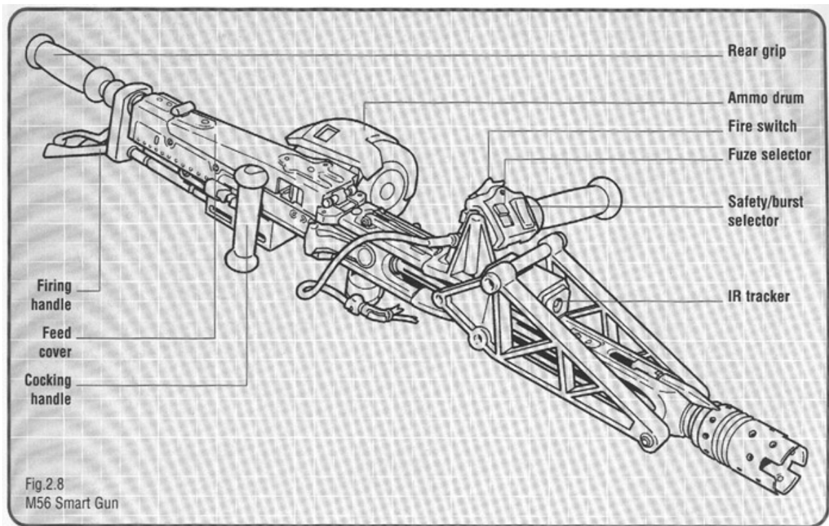
Colt M56 Smartgun
